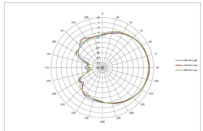
5 GHz antenna patterns (vertical)
