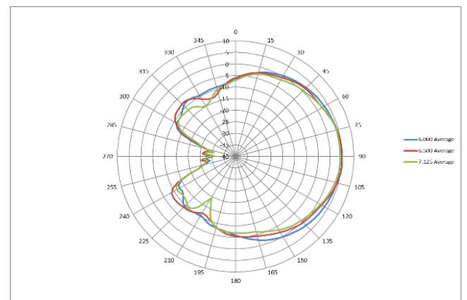
6 GHz antenna patterns (vertical)
