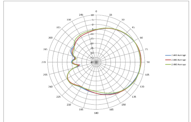
2.4 GHz antenna patterns (vertical)
