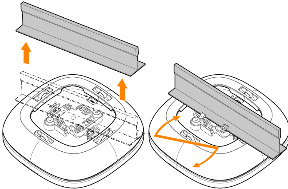
Figure 2 Installing the Access Point (with Sleeve) to a Ceiling Rail
