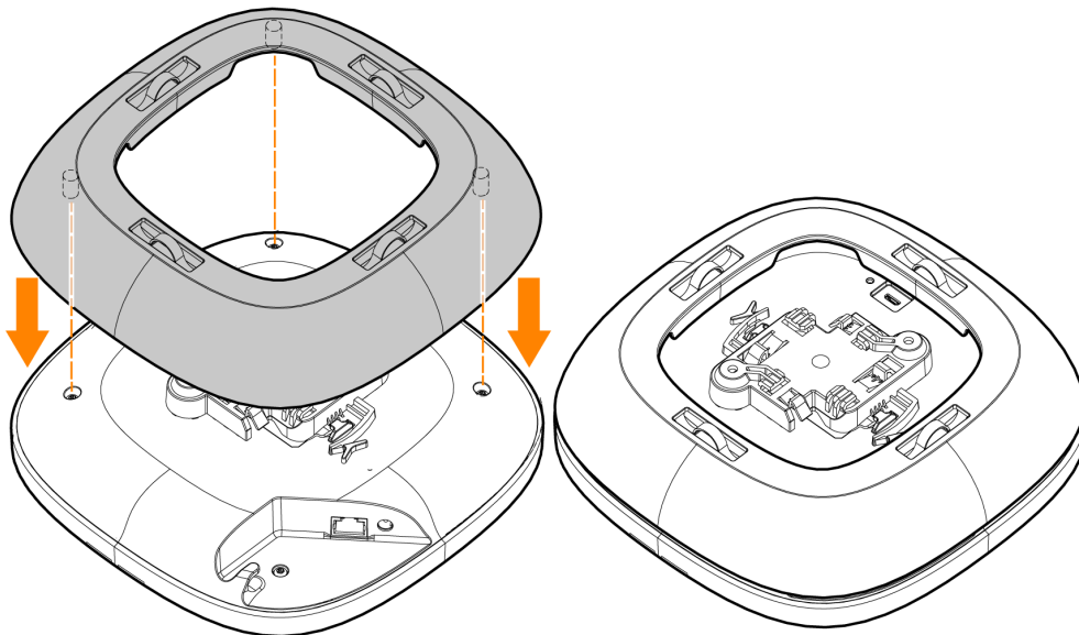
Figure 1 Attaching AP25 Flush Mount Sleeve onto access point
