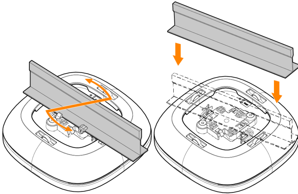
Figure 3 Removing the Access Point (with Sleeve) from a Ceiling Rail
