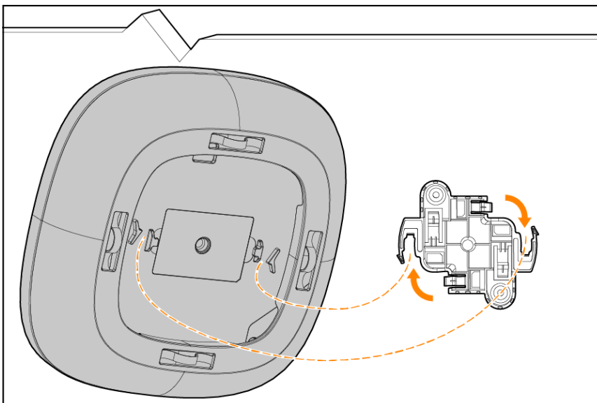
Figure 4 Installing the Access Point (with Sleeve) to a Wall
