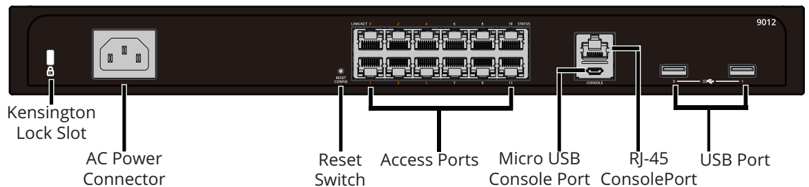
Figure 2 Back Panel of the HPE Aruba Networking 9012 gateway
