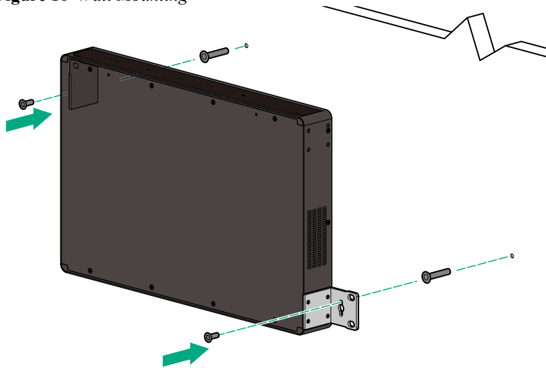
Figure 10 Wall Mounting
