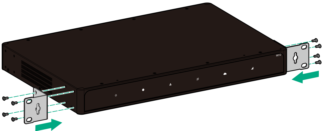
Figure 6 Rack Mount Bracket
