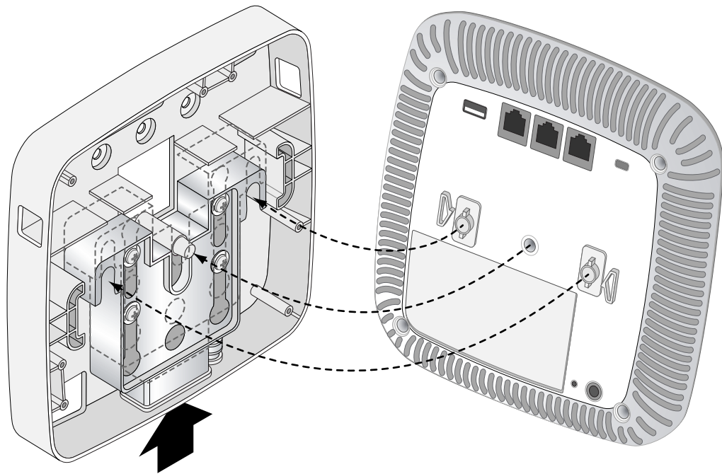
Figure 5 Attaching the AP to the Mounting Bracket
