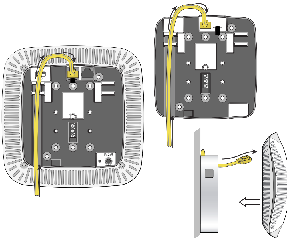
Figure 1 Ethernet cable from below the AP
